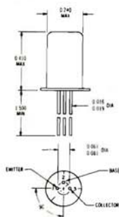
TO-12 CASE 34A
